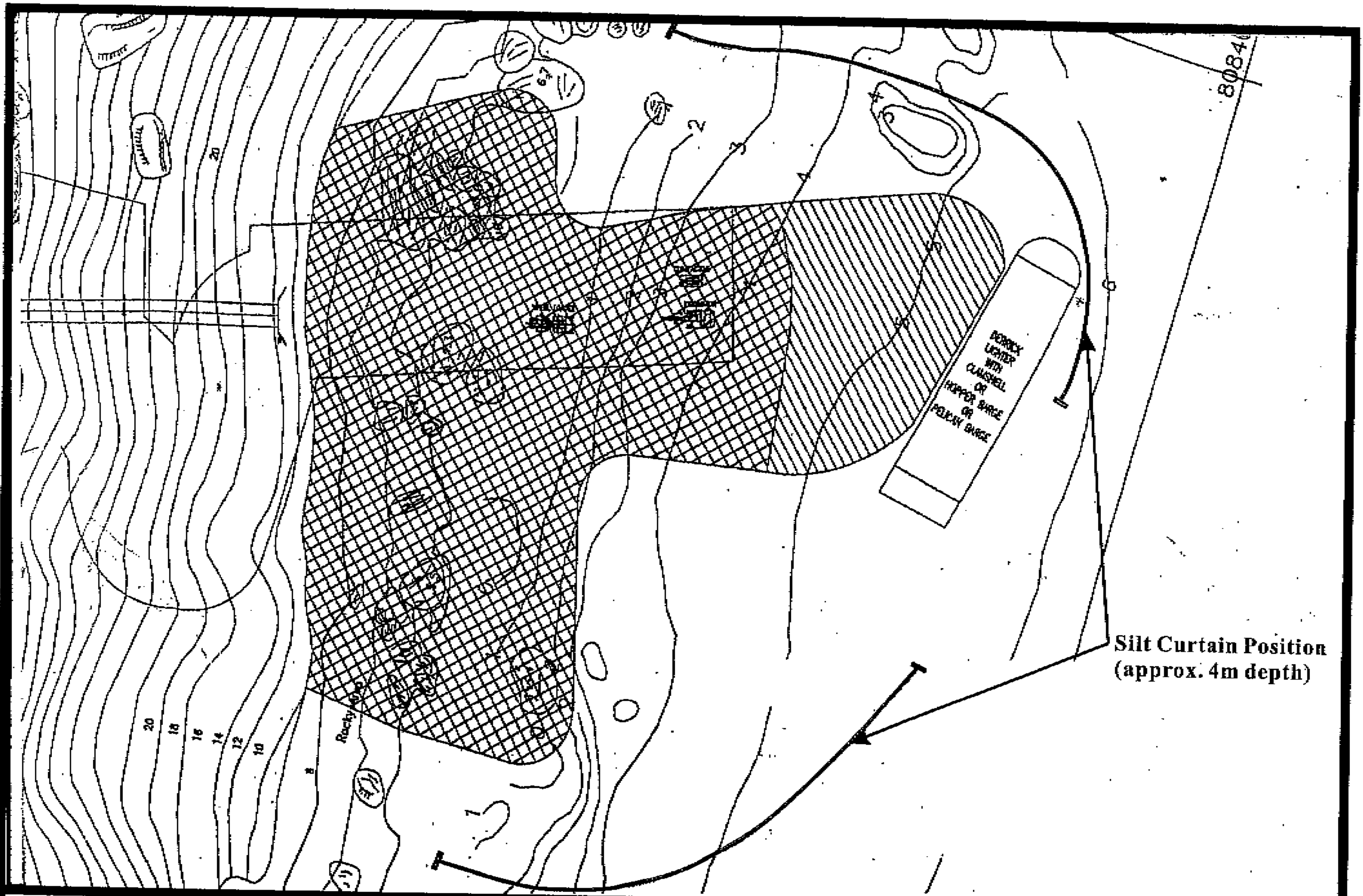
Figure 7 Location of Silt Curtain Installation at Tai Long Wan
